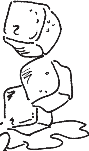
SOLID (ice)
